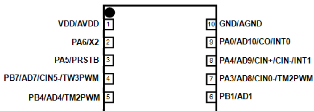
PFS172-4N10 (DFN3*3-10pin-0.5pitch)
