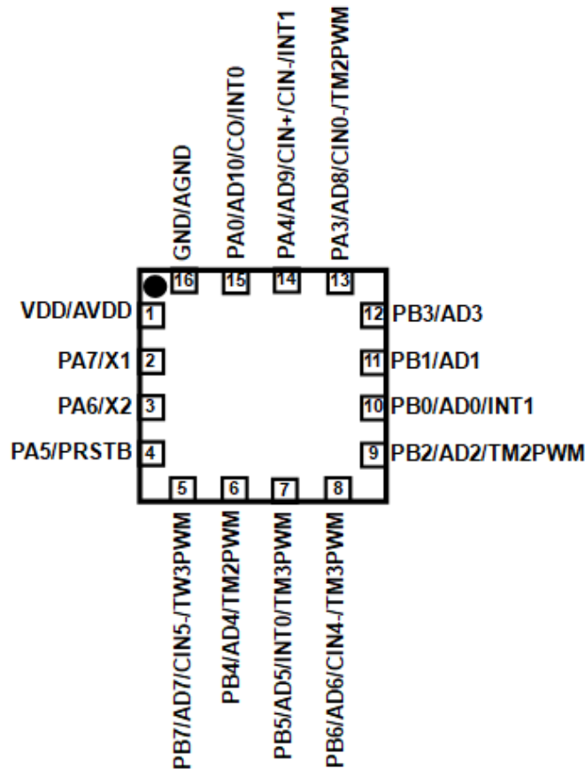
PFS172-1J16A (QFN3*3-16P-0.5pitch)
