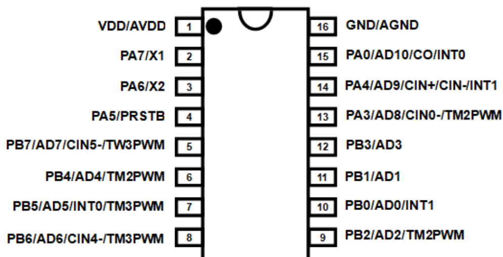
PFS172-S16A (SOP16-150mil)
