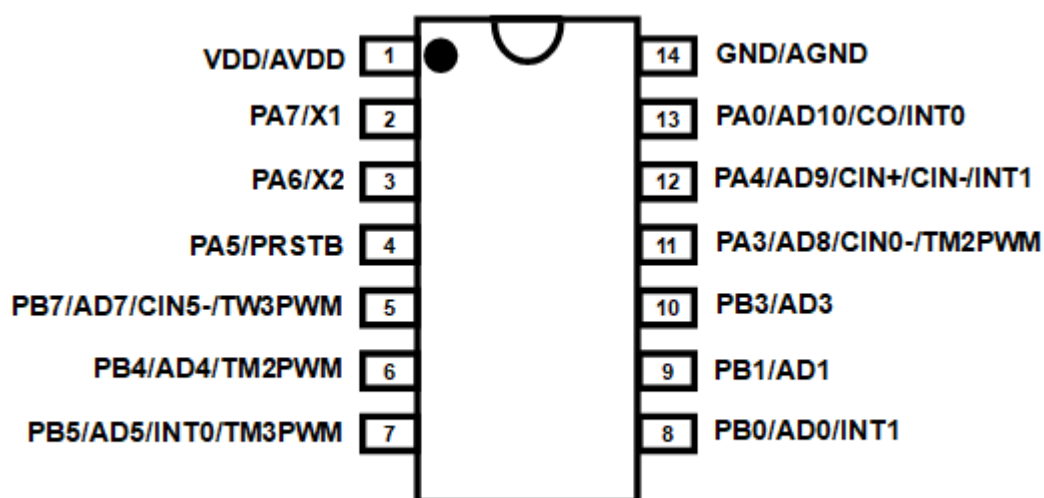
PFS172-S14 (SOP14-150mil)
